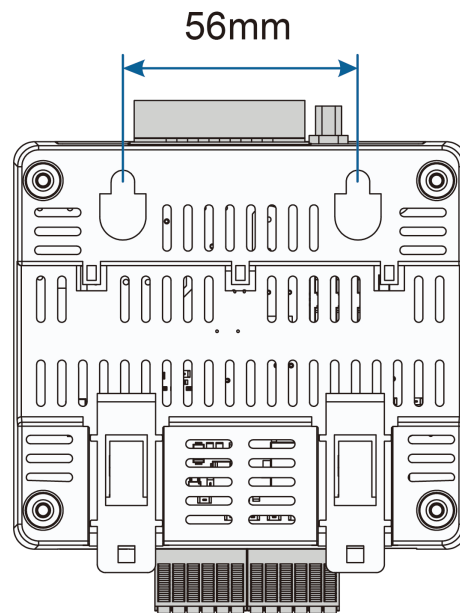
figure 5-1 Mounting Holes
