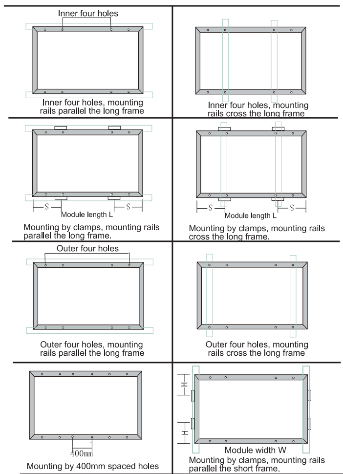
Figure 4 Installation Methods
